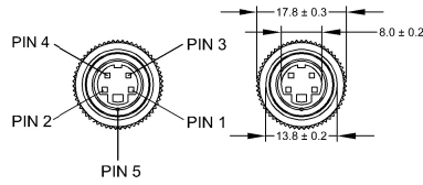
4 PIN FEMALE MATING FACE
